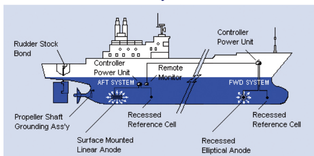
Typical Layout of Impressed Current Cathodic Protection System
