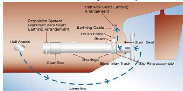
The layout of the shaft earthing & monitoring assembly
